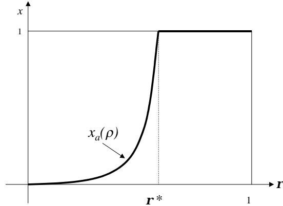
Figure 3: Self-restraint in the single-agent case
