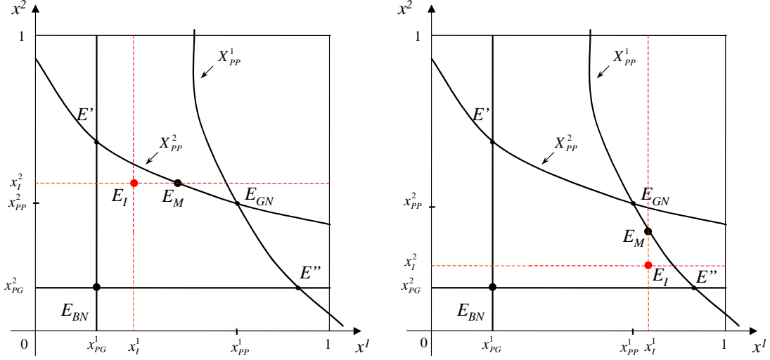
Figure 8: Mixed, Extreme News, and Bad News equilibria
