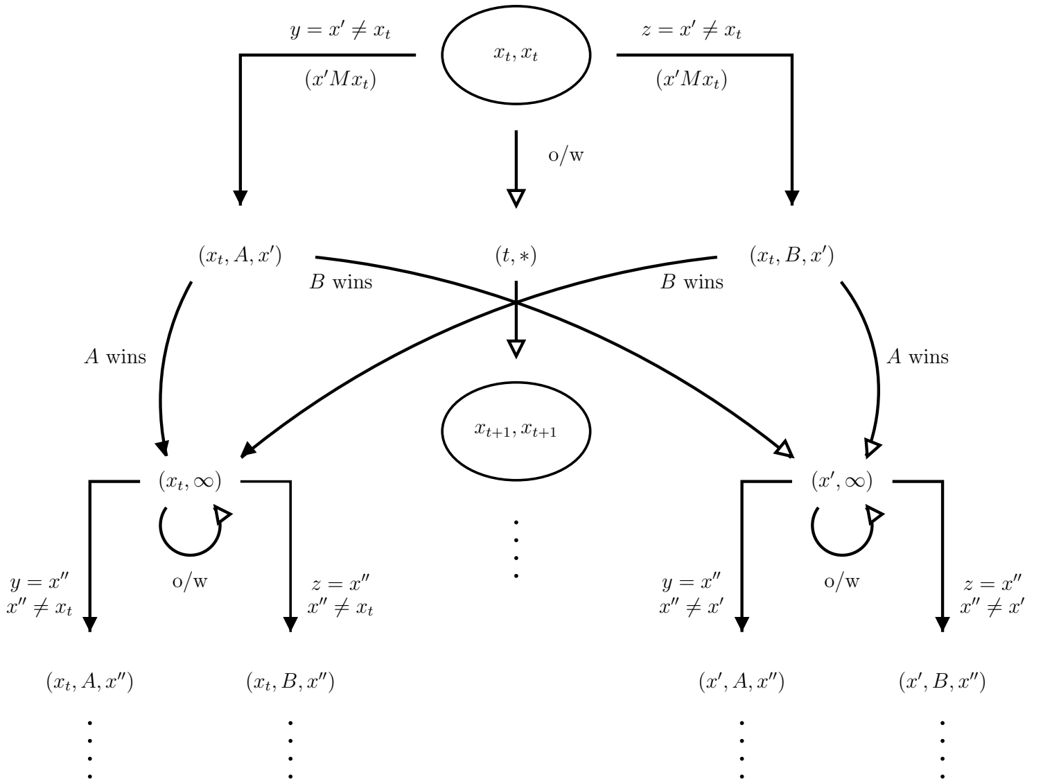
Figure 1: States in the proof of Prop. 2
